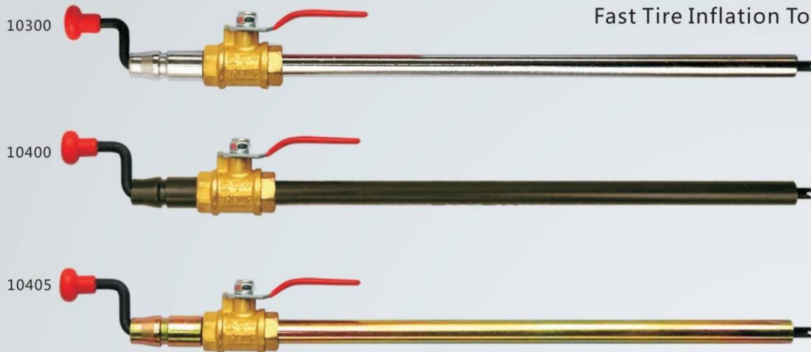
10300 快速充气装置-28cm镀铬 Fast Tire Inflation Tool (28cm Chromium plated)
